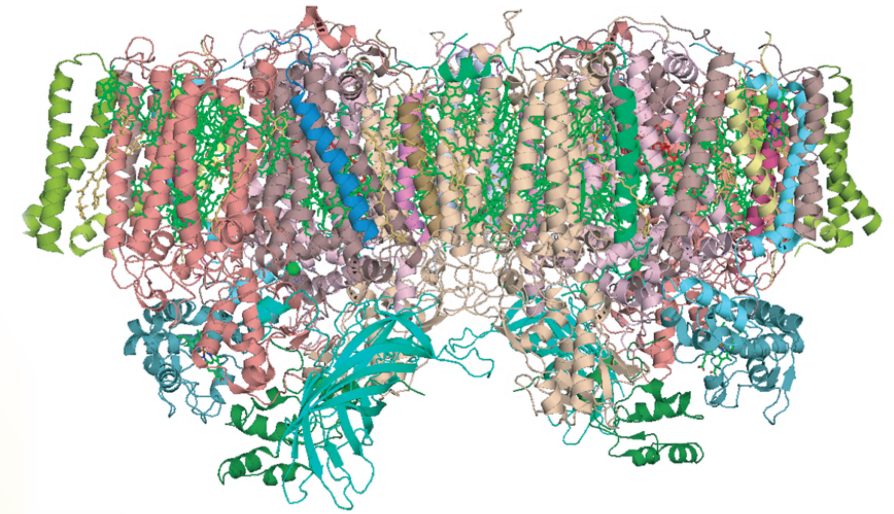
Figure 1: Photosystem II protein.
